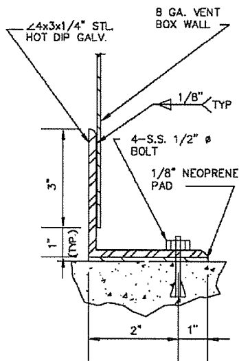
SECTION B-B
