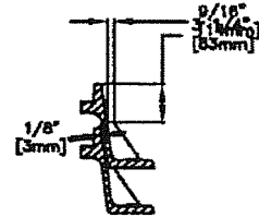
STACK DETAIL
