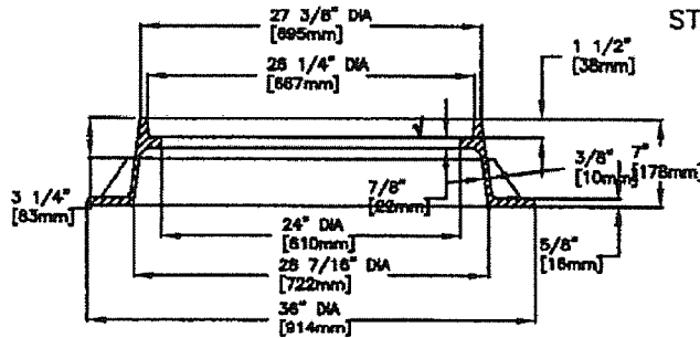
FRAME SECTION
