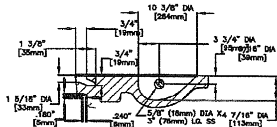
GROOVE, PICKHOLE, PICKBAR DETAIL
