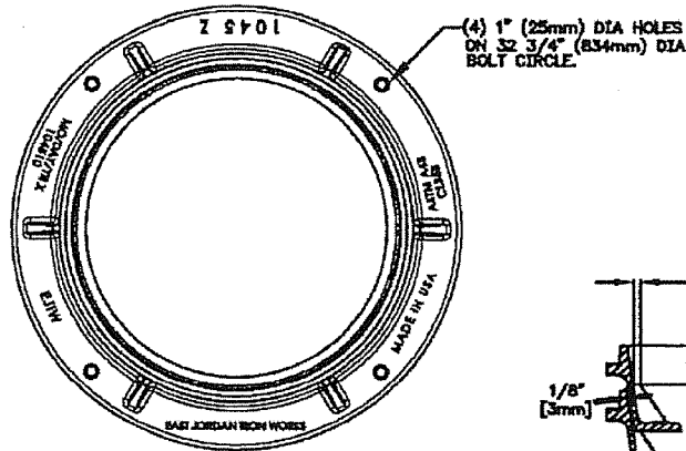
STACK DETAIL
