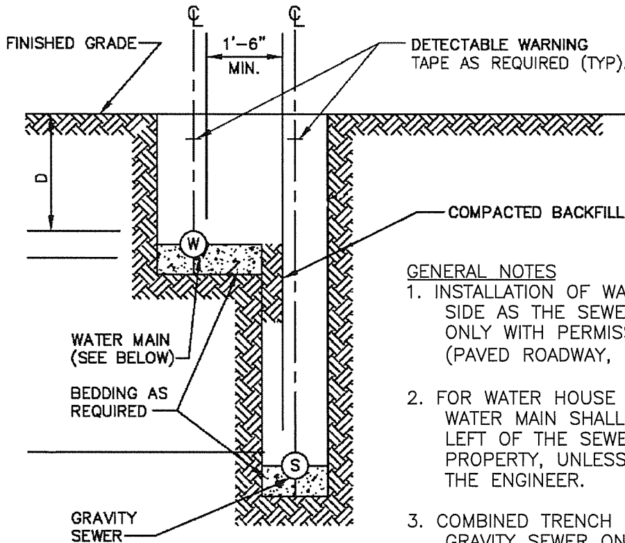
OPTIONAL SECTION (COMBINED TRENCH)
