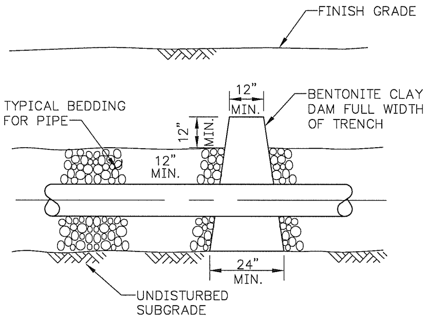
CLAY DAM DETAILS
