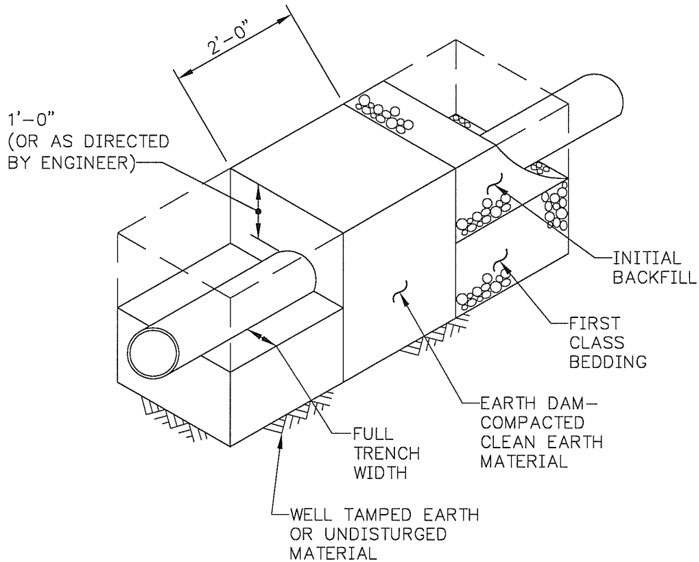
EARTH DAM DETAIL
